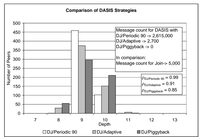
Figure 3. This graph shows the comparison of the minimal depth join algorithm using the three described DASIS approaches— periodic DASIS with an update interval of 90 time units, adaptive DASIS , and piggyback DASIS . The simulation started with an initial P2P system containing two peers and inserted 561 peers. This leads to an optimal depth of 9.
