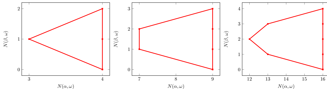
Figure 1: Examples of three relational marginal polytopes given by the first-order logic formulas \alpha = sm(x) \wedge fr(x, y) \Rightarrow sm(y) and \beta = sm(x) for domains of size 2, 3 and 4.
