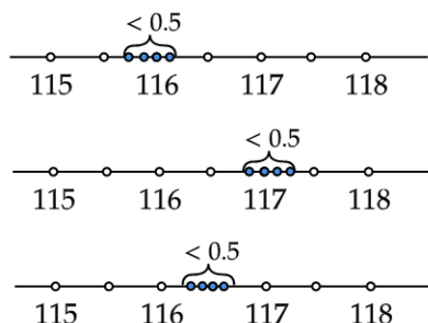
■ Figure 2 A few examples of possible outputs obtained in \Pi_{AA} . In the top and middle examples, representing cases (a) and (b) respectively, honest outputs are close to a single integer. In the bottom example, representing case (c), some honest outputs are closer to 116, while some are closer to 117.
