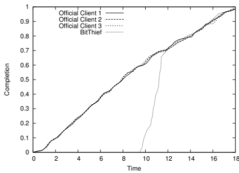
Figure 4: Download times for three official clients and one BitThief client in the presence of a slow seeder. BitThief starts downloading 9 minutes later than the other clients, but catches up quickly. Ultimately, all clients finish the download roughly at the same time.
